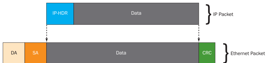
Figure 8. IP framing inside Ethernet.
