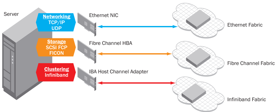
Figure 5. A traditional deployment model requires three separate network interface cards (NICs).
