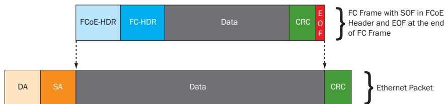
Figure 7. Fibre Channel framing inside Ethernet.
