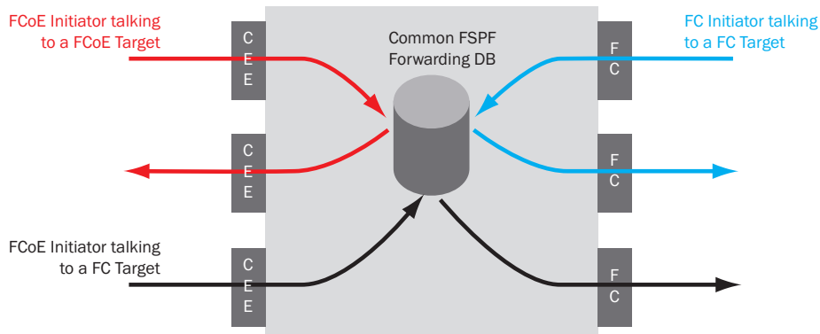
Figure 9. FCoE switch supports Fibre Channel traffic between CEE ports and between Fibre Channel ports and CEE ports.
