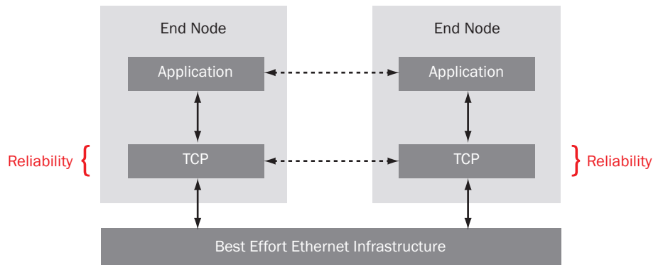
Figure 2. Reliability in end points for TCP/IP applications which wastes processing cycles and hinders application performance.
