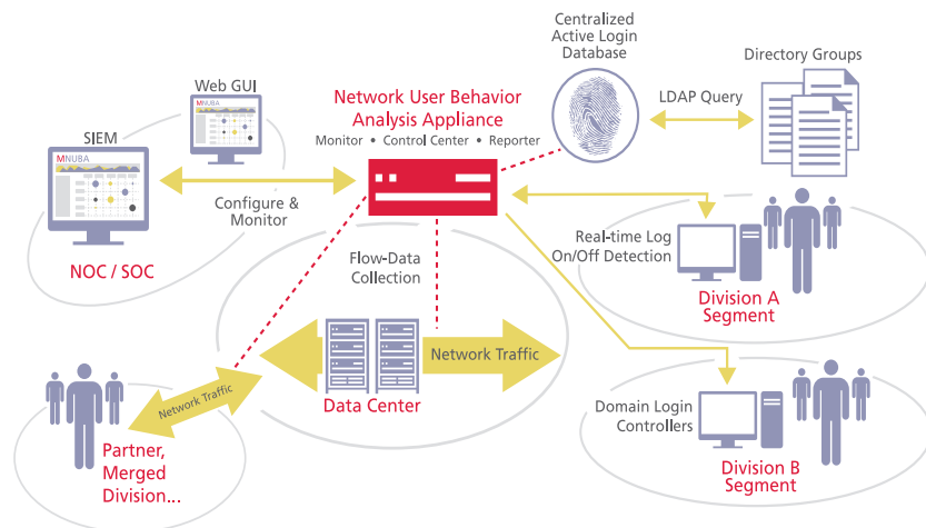
Representative McAfee Network UBA Control Center and Monitor appliances deployed in front of a data center where critical business systems reside.
